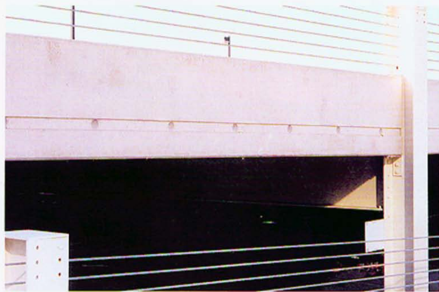
Close up of the P/T anchors showing how the deck, the P/C panels and the steel columns work in a composite manner
